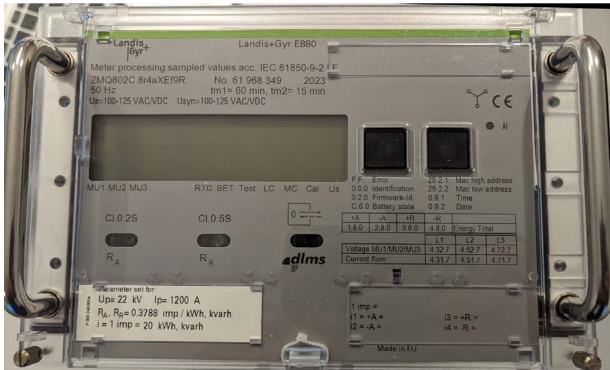
Figure 15 Energy meter from Landis+Gyr.
