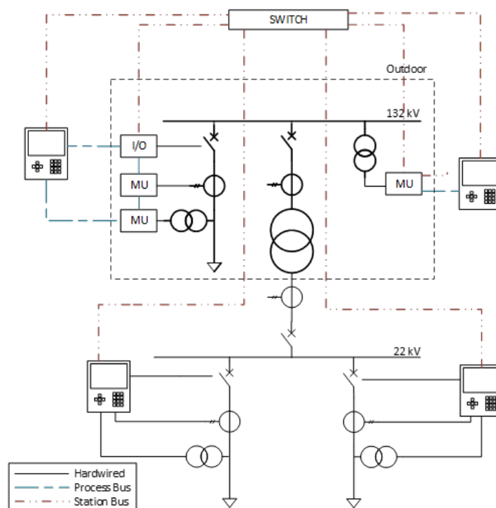
Figure 6 Simplified topology for Tørdal Substation
